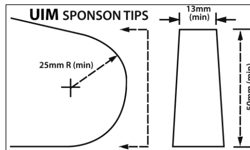
Figure 4 - UIM Sponson Tips
